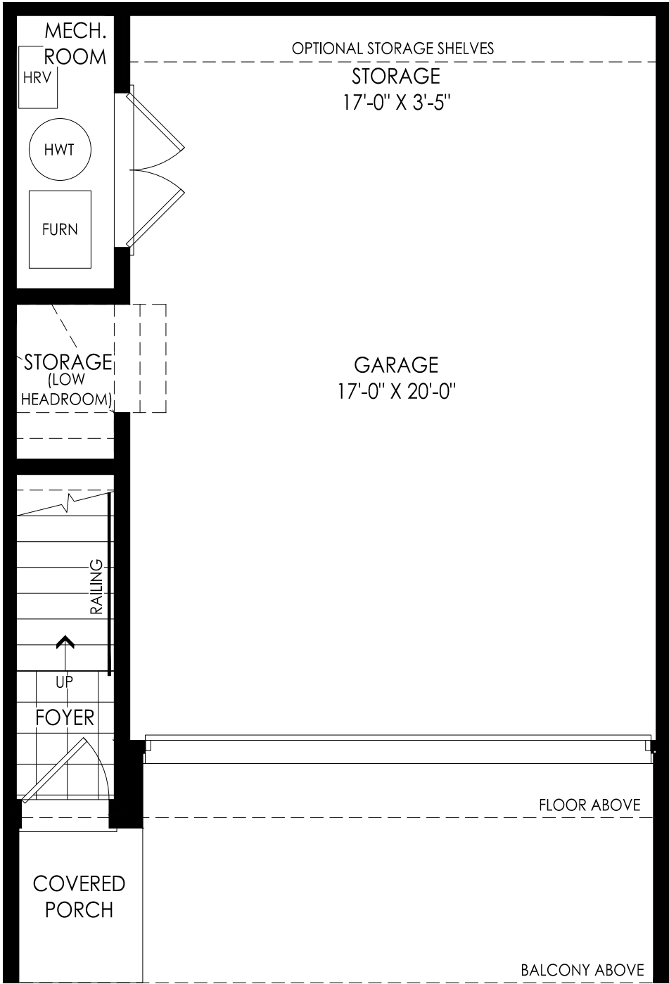
GROUND FLOOR ELEV. A/B
